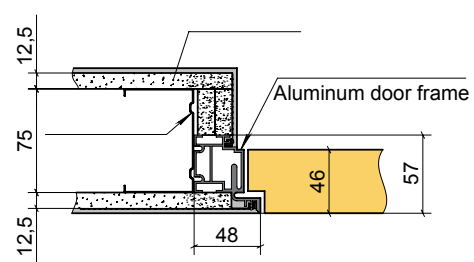
Aluminum door frame iDoors "INSIDE" reverse opening
