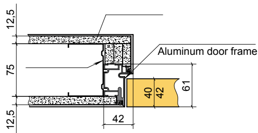
Aluminum door frame iDoors "Standard" external opening
