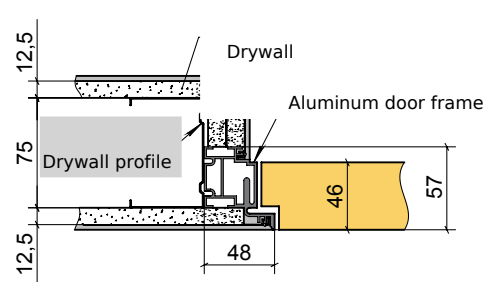
Aluminum door frame iDoors "INSIDE" reverse opening
