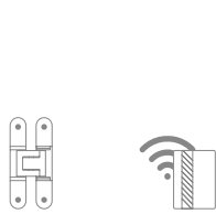
Concealed hinges Recessing for electronic lock
