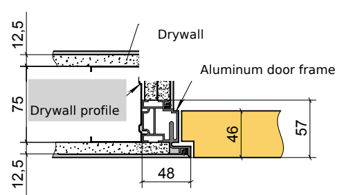
Aluminum door frame iDoors "INSIDE" reverse opening
