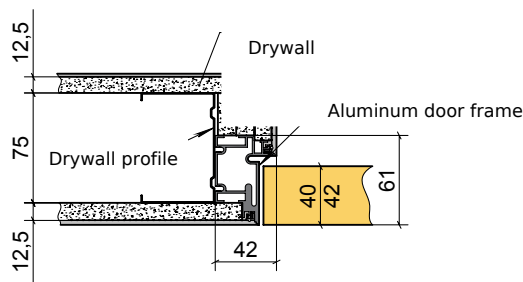
Aluminum door frame iDoors "Standard" external opening
